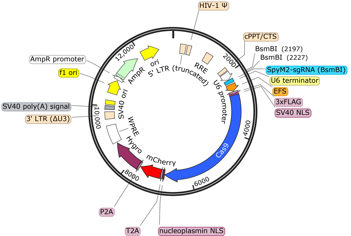
pBC2101-eci_wtCas9-with-NLS_lenti
