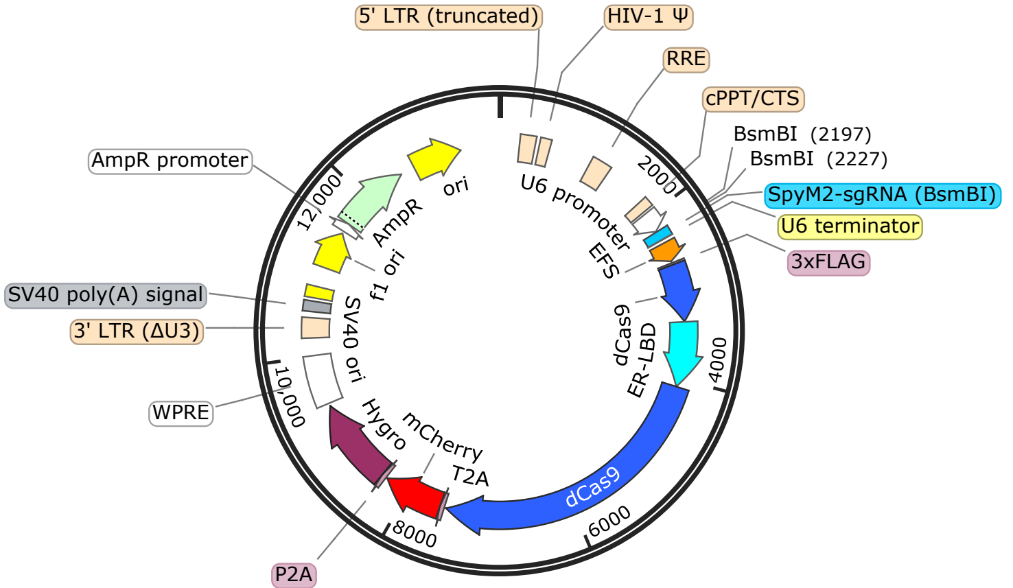
pBC2103-eci_arCas9-without-NLS_lenti
