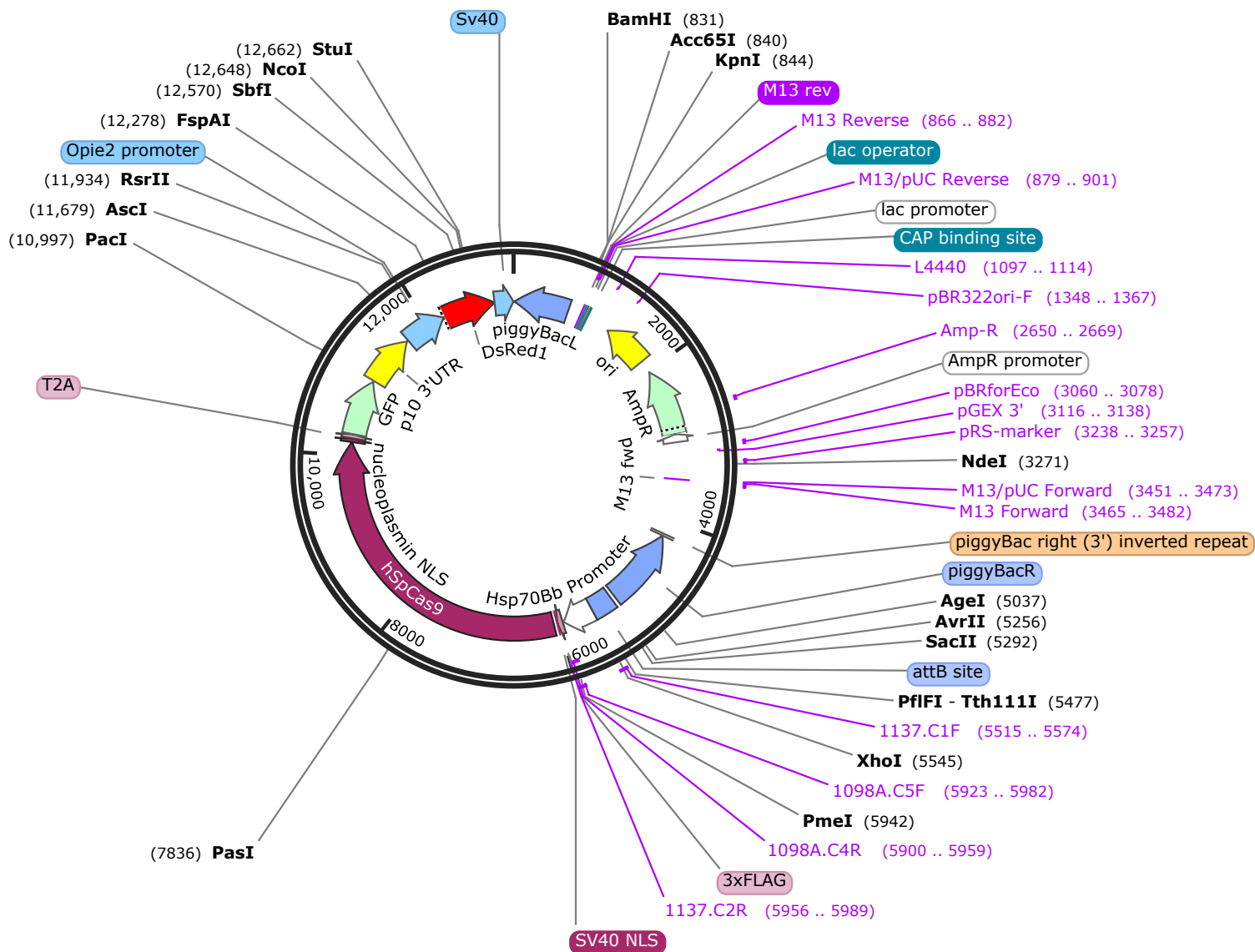
1137=DmelHsp70Bb-Cas9 13,159 bp
