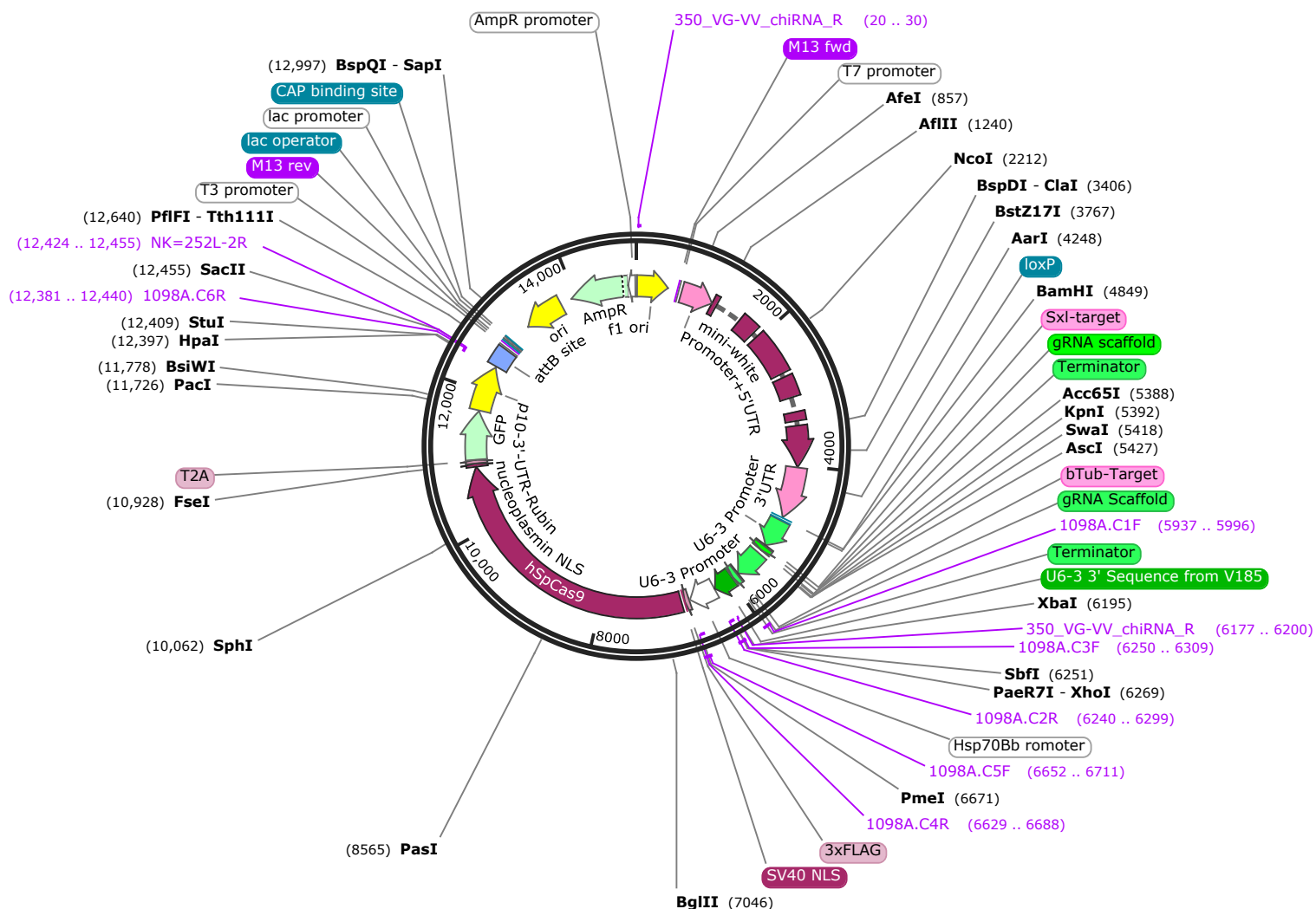
1098A=one-locus pgSIT[sxl,bTub,Hsp70Bb-Cas9] 14,921 bp
