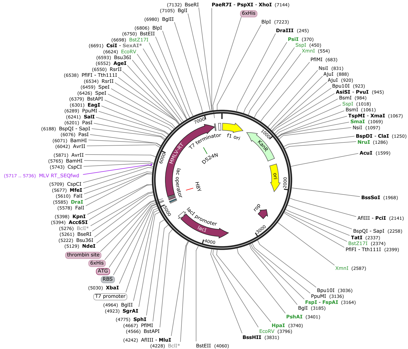
pET-28a_6H-MMLV_RT_D524N-6H 7306 bp
