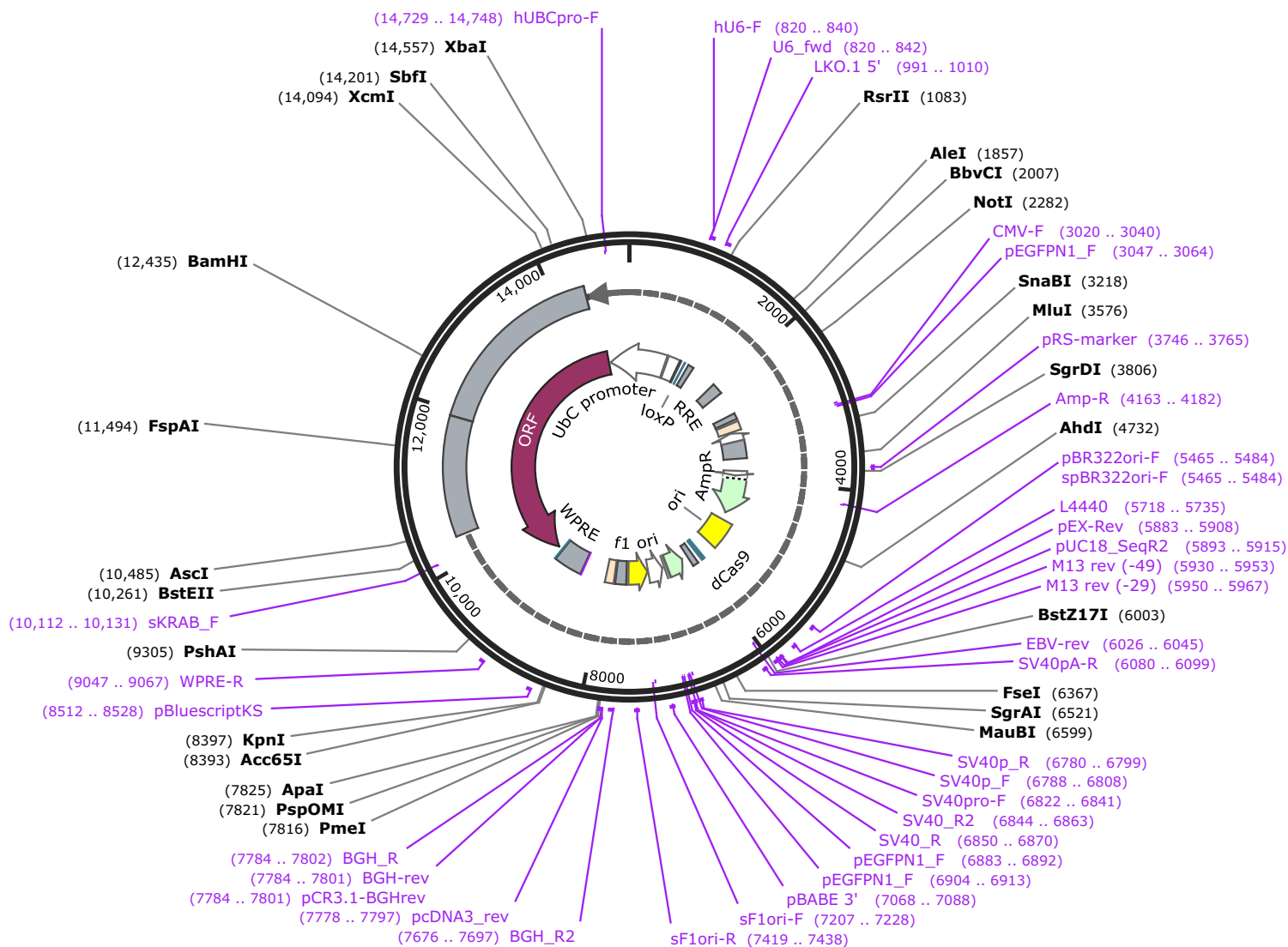
AAAA-0245-pLV-RnSyt1-sgRNA1-dCas9-KRAB-TagBFP 15,009 bp
