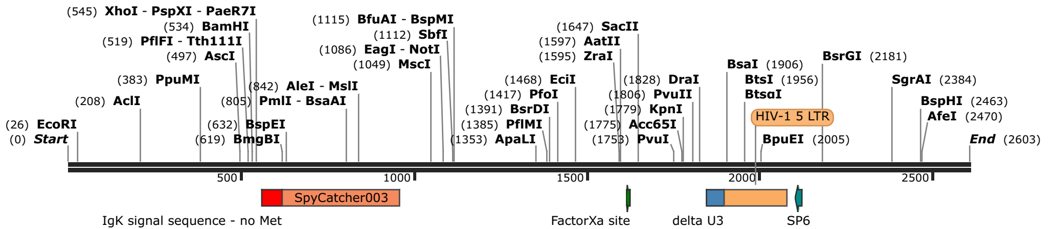
phr-sin-bx_igk_spyc003_hcd52_insilico-txt 2603 bp
