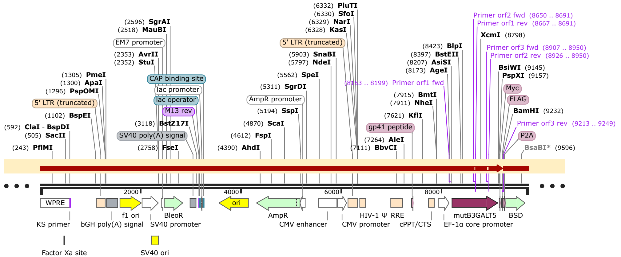
lentiMutB3GALT5-blast_D156A_D243A 9719 bp
