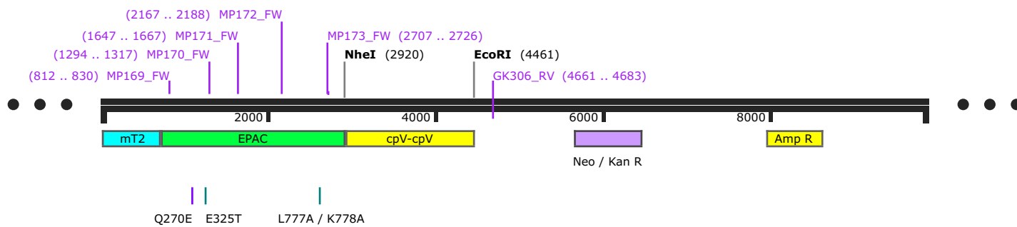
H325_mTurq2del_EPACdDEPCD_Q270E_E325T_L777A_K778A-tdcp173V(ST) 9846 bp
