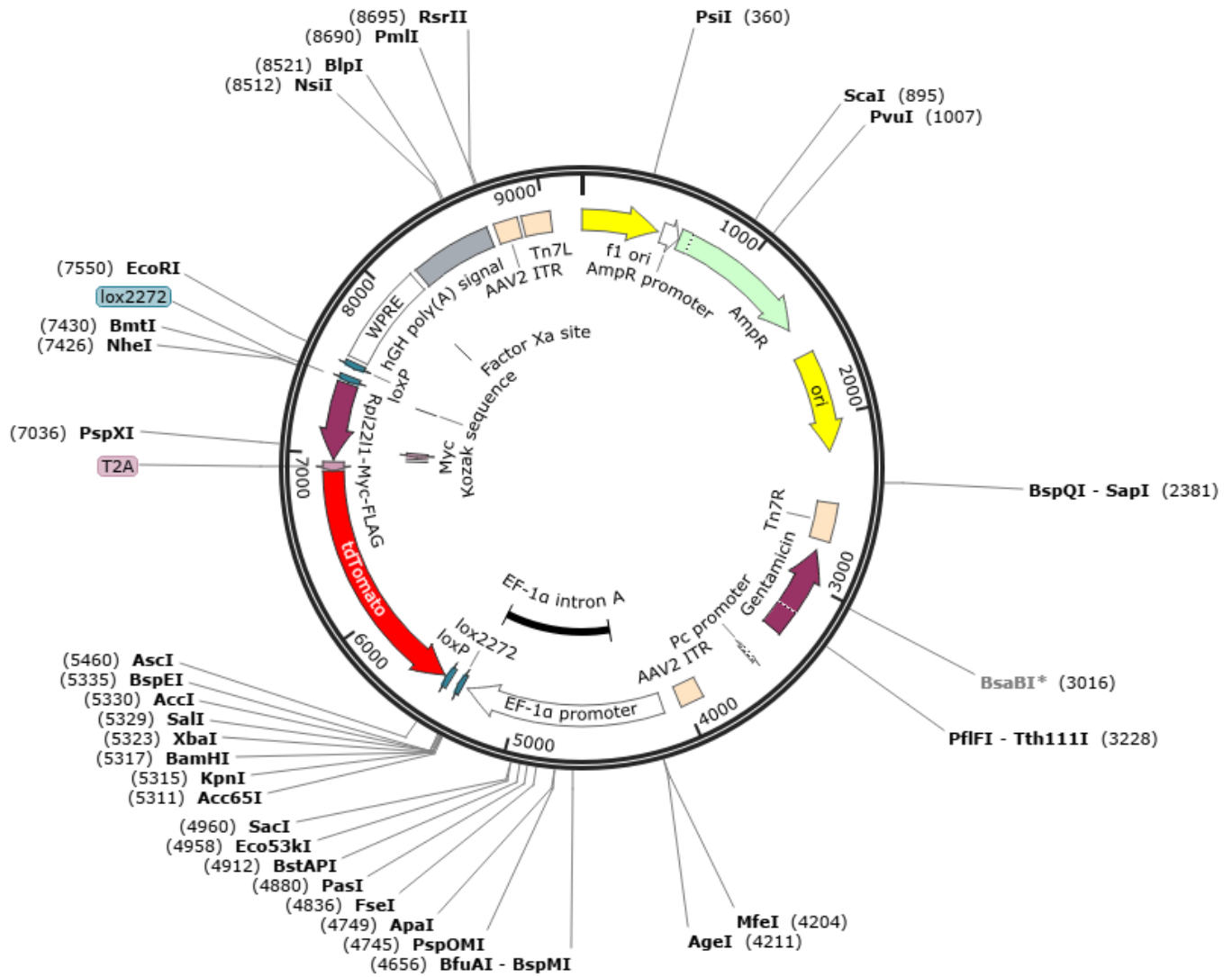
pFB-EF1a-DIO-Rpl22l1-myc-FLag-2A-tdTomato-WPRE-hGHpA 9221 bp
