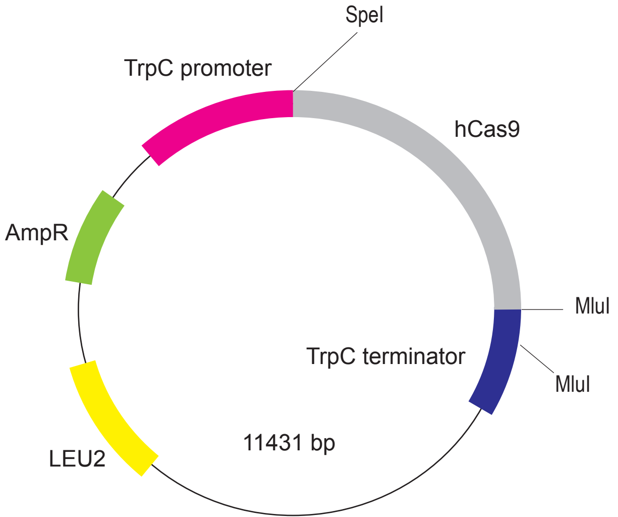
p415-PtrpC-Cas9-TtrpC-CYC1t
