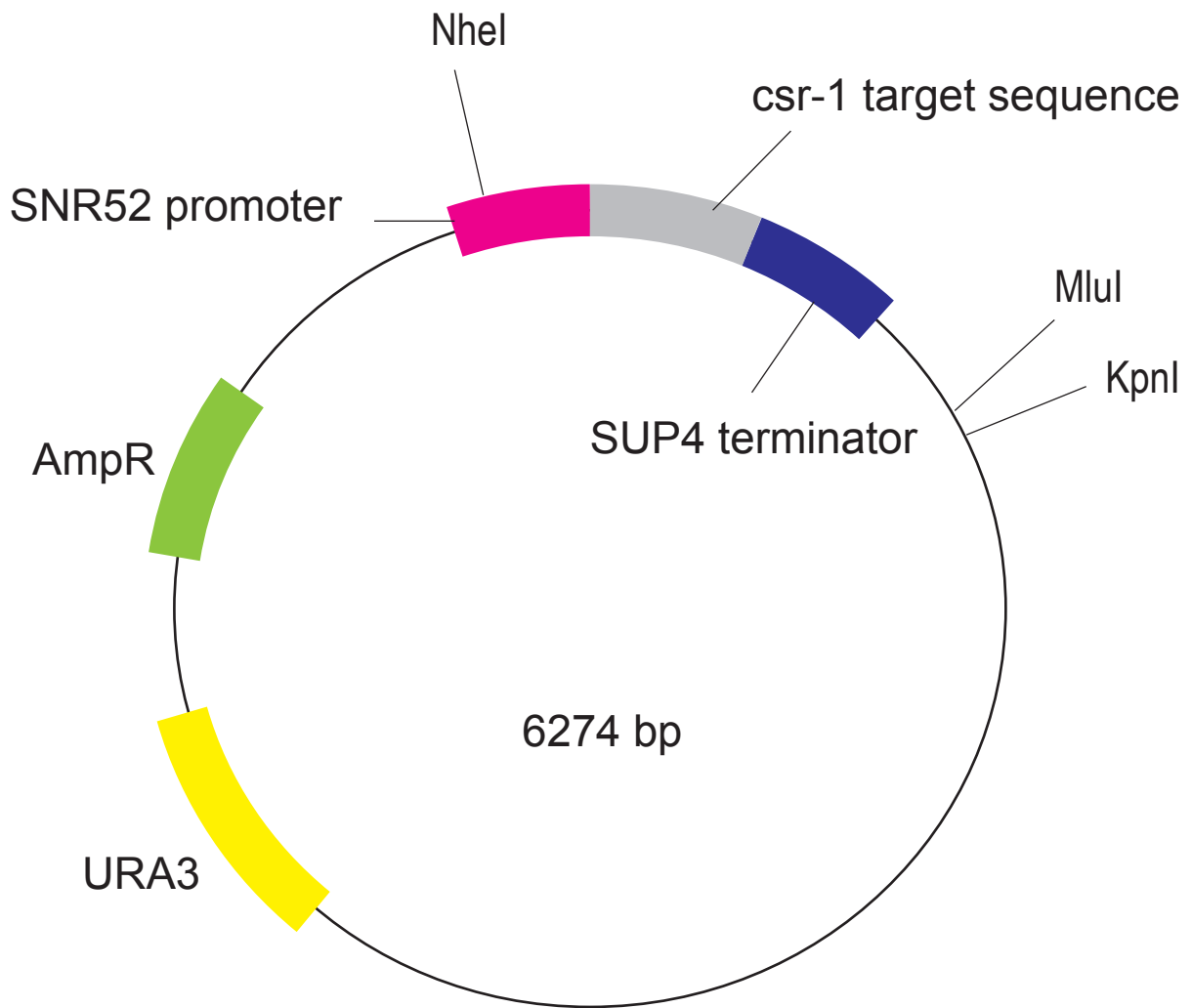
p426-SNR52p-gRNA.csr-1.Y-SUP4t
