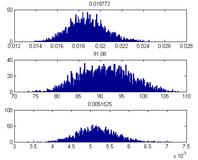
superfolder GFP mature protein parameter distributions
