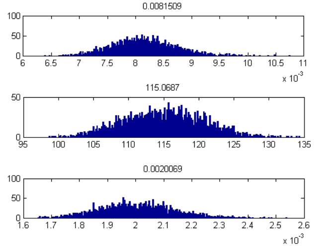
superfolder GFP mature protein parameter distributions
