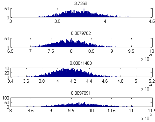
superfolder GFP total protein parameter distributions
