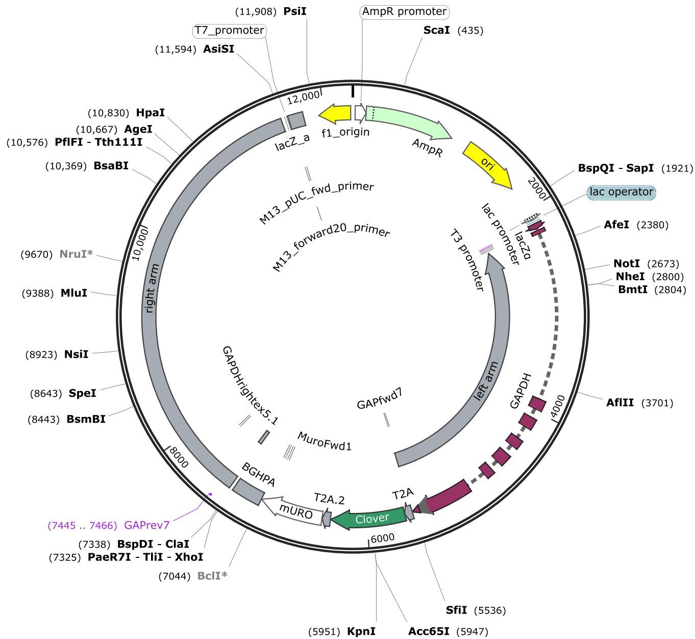
GAPTrapT2ACloverT2AMuopABGH_Addgene_Submission 12,273 bp
