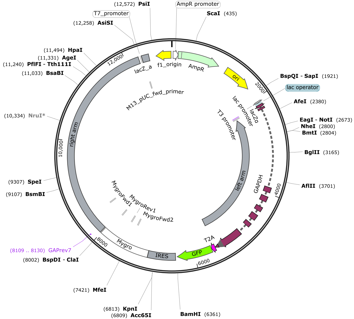
GAPTrapT2AeGFPiResMygro_Addgene_Submission 12,934 bp
