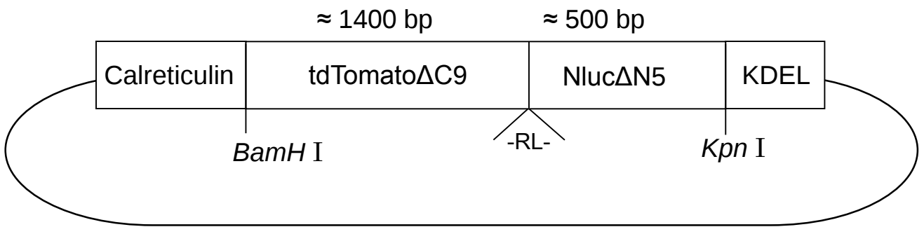
pcDNA3-Calreticulin-ReNL-KDEL
